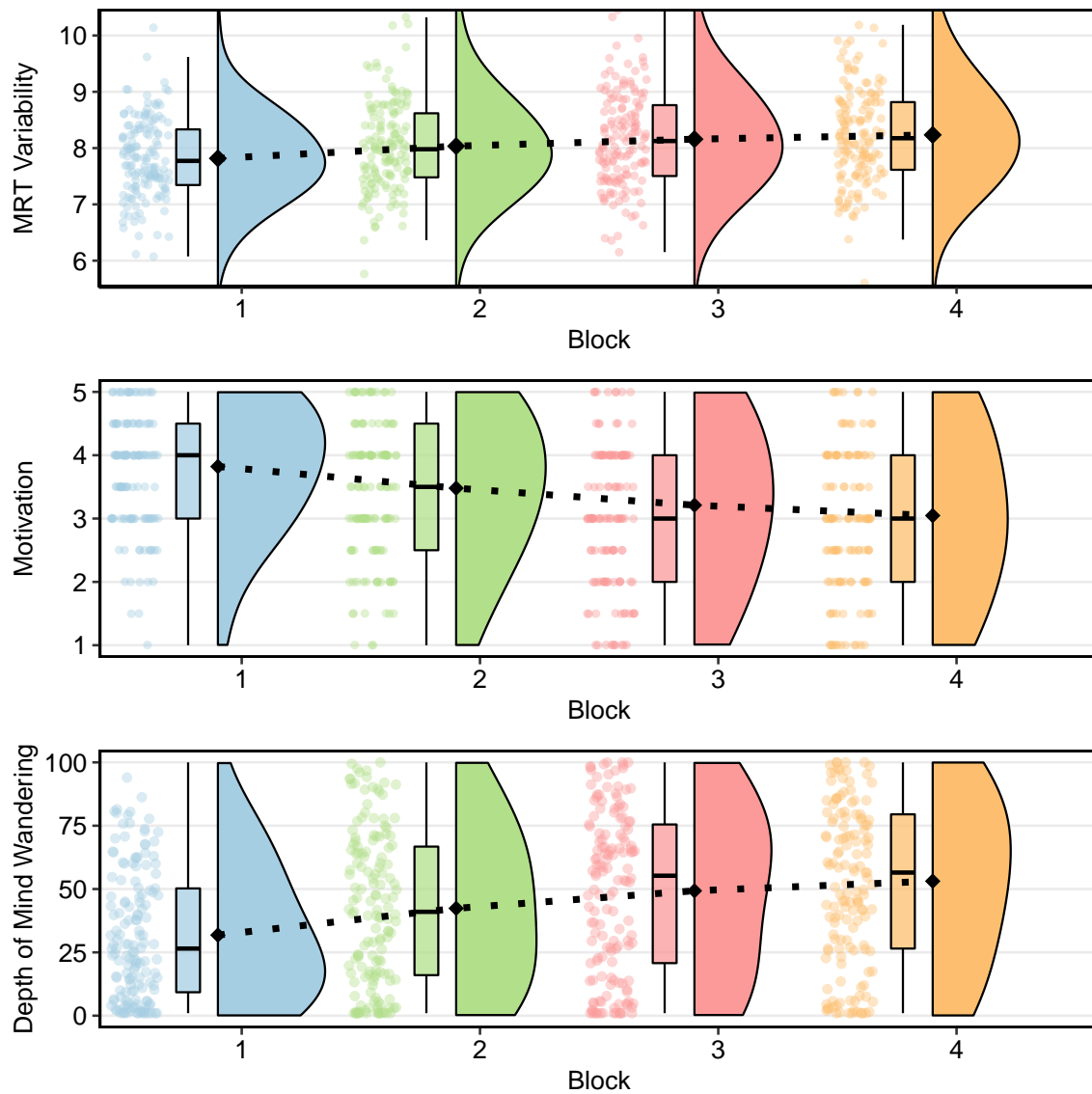
Figure 1. Distributions of participant data for metronome response task (MRT) variability, motivation, and mind wandering, plotted across trial blocks.
